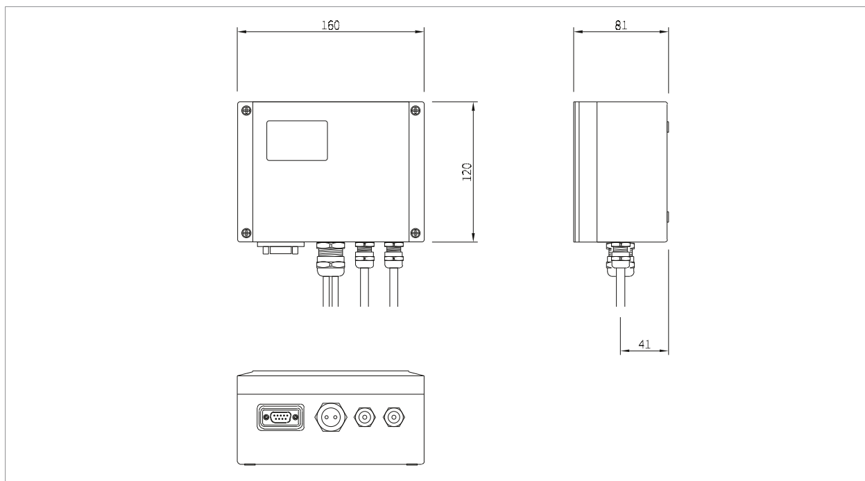
USCX100 (dimensions in mm)
